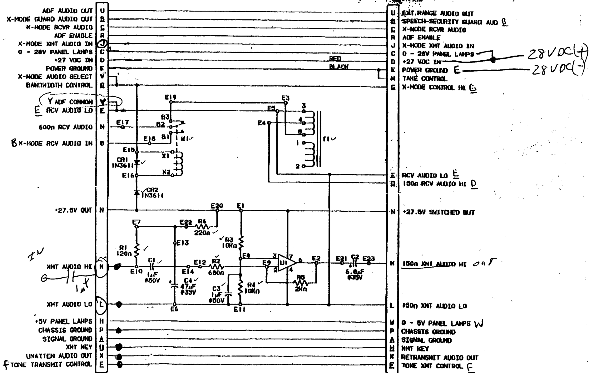
WIRING FIGURE
